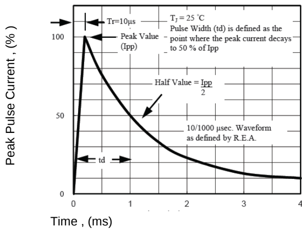
Fig 5 Pulse Waveform
